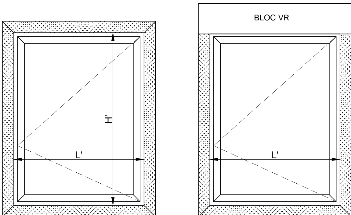
ELEVATION INTERIEURE
